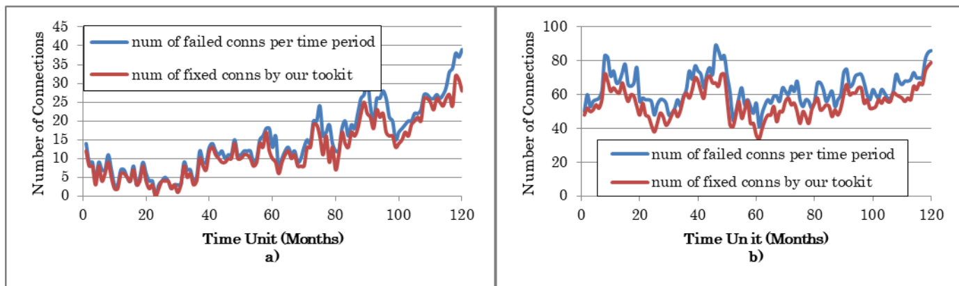
Fig 6. Evolution of the number of failed and repaired connections due to aging in the network for a) 20Tbps and b) 49.2Tbps initial loads.
