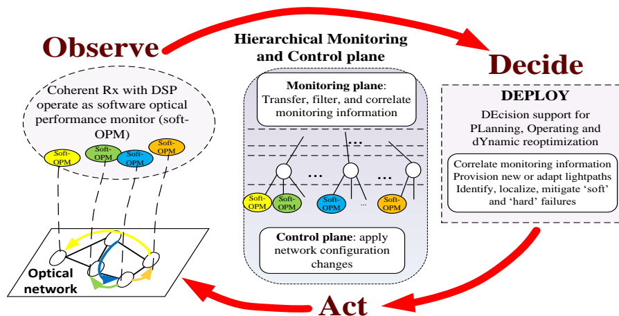
Fig. 1: The ORCHESTRA observe-decide-act control cycle.
