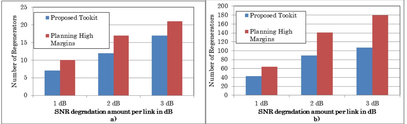
Fig 4. Number of regenerators required as a result of a single link soft failure of 1, 2 and 3 dB for a) 20Tbps and b) 49.2Tbps loads.
