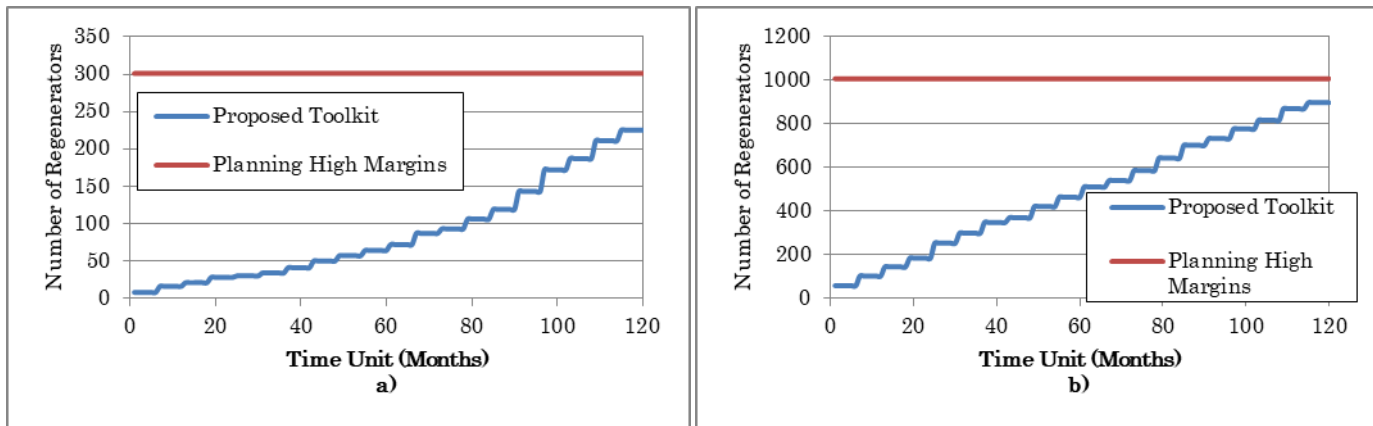
Fig 5. Evolution of the number of regenerators required as a result of network aging for a) 20Tbps and b) 49.2Tbps loads.
