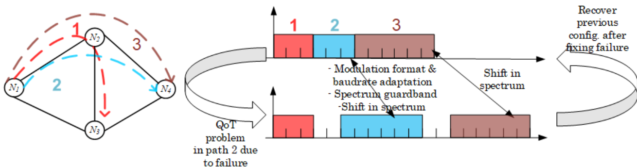
Fig 2. Paths 2 and 3 are shifted in order to create guardbands and assign more slots to increase baud rate and decrease mod format of path 2. After the failure is identified and fixed, the network can return to the original state.
