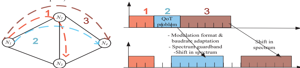
Fig 1. Paths 2 and 3 are shifted in order to create guardbands and assign more slots to increase baud rate and decrease mod format of path 2
