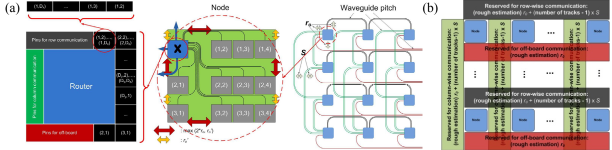
Figure 1: (a) Node layout and pin allocations of the router for router chips with peripheral pinout and (right) a 2-D grid array ( 3 \times 4 ) lay-out of 3 \times 2 \times 2 mesh on-OPCB; (b) Lay-out design rules on 2D grid for OPCBs. Space reserved for row-wise, column-wise and off-board communication.
